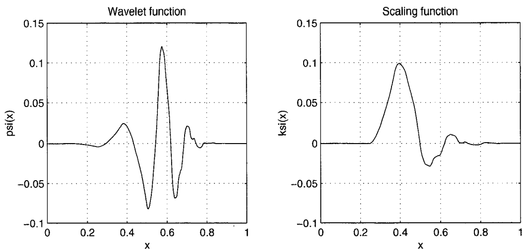
FIGURE 2.10. Daubechies family wavelet and scaling function, M=8 .
