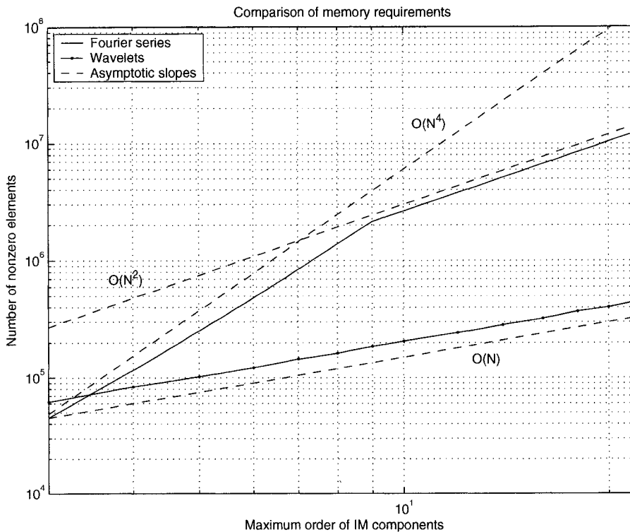
FIGURE 3.28. Number of nonzero elements in the Jacobian for Gilbert cell mixer in Fig. 3.24.
