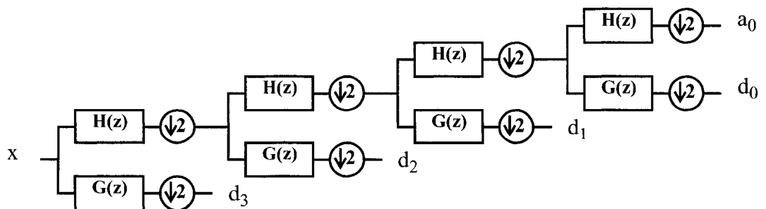
FIGURE 2.15. Wavelet decomposition tree.
